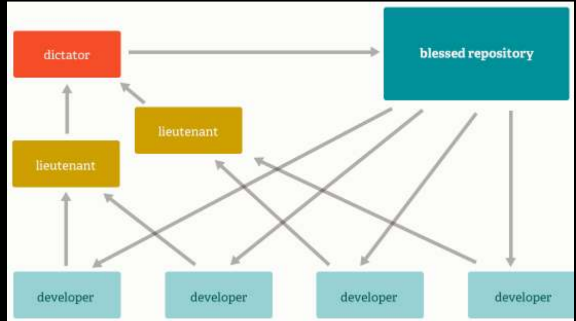
Dictator and Lieutenants Workflow
